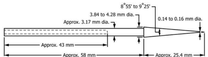
FIG. 2 Standard Needle
